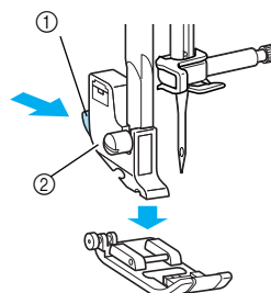
② Support de pied-de-biche
